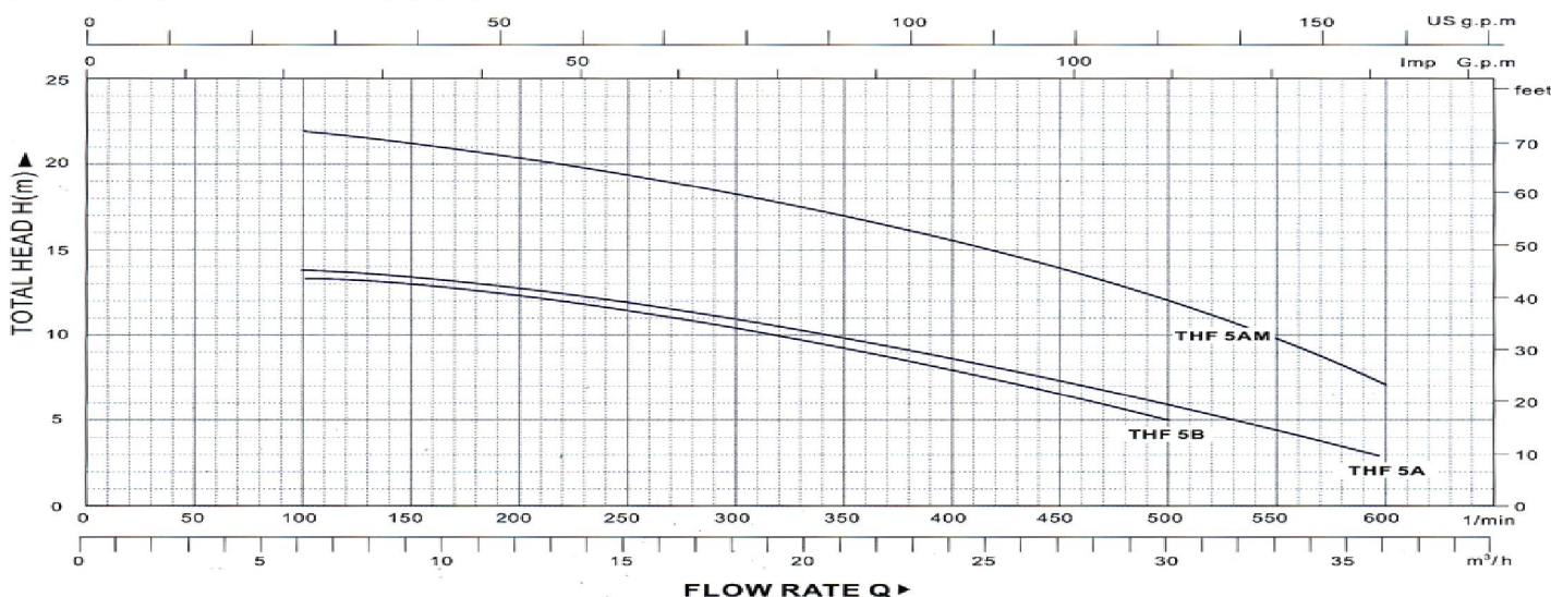
PERFORMANCE CHART AT n=2900 l/min
